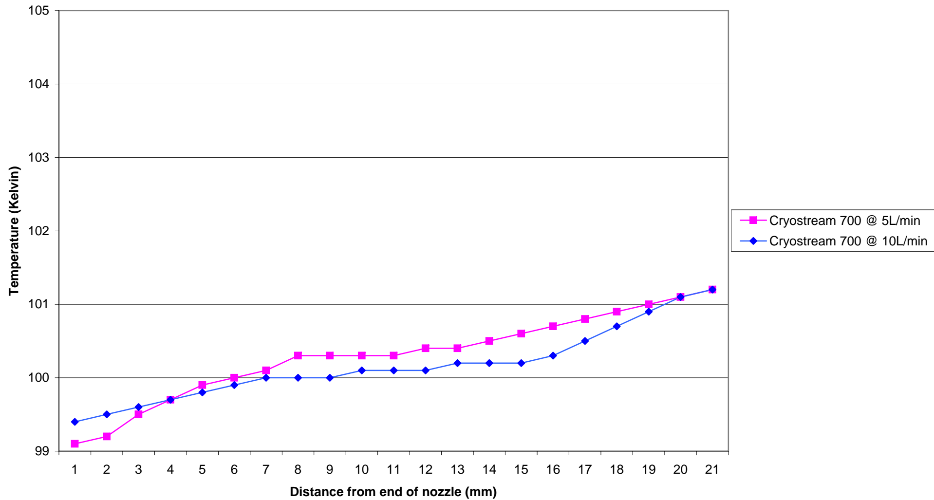
Distance from end of nozzle v. gas temperature at a set point of 100.0K
